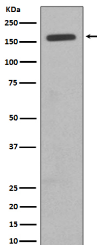
Western blot analysis of CD11b expression in TF1 cell lysate.
